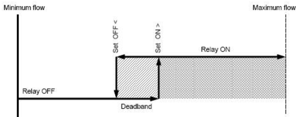
Fig 4.2 Single Point Alarm Operation
