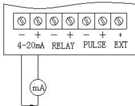
Fig 2.3 4-20mA
