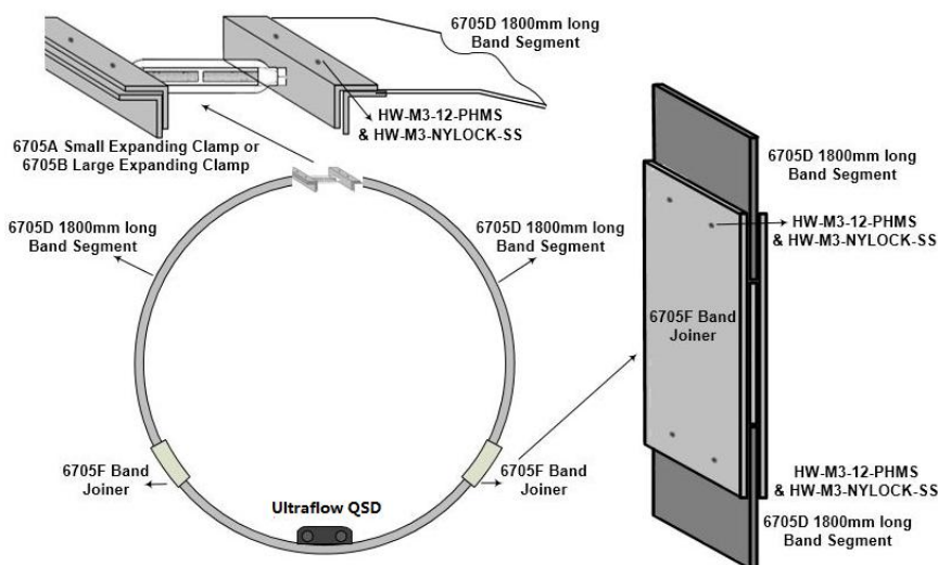
Figure 5.5. Model 6705 Expanding Band Kit
