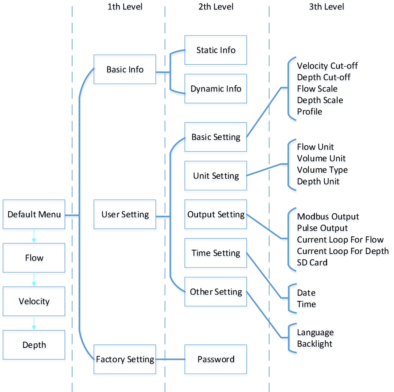
Figure 6.2 Menu Structure
